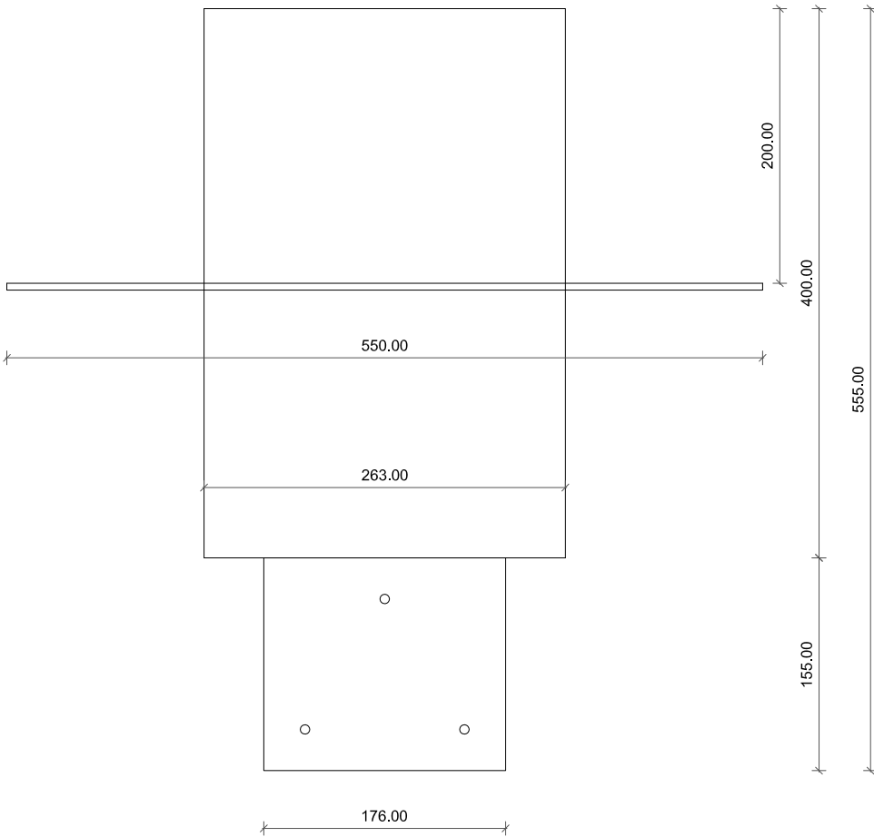
○ Ceiling Bracket Scale - 1:5
